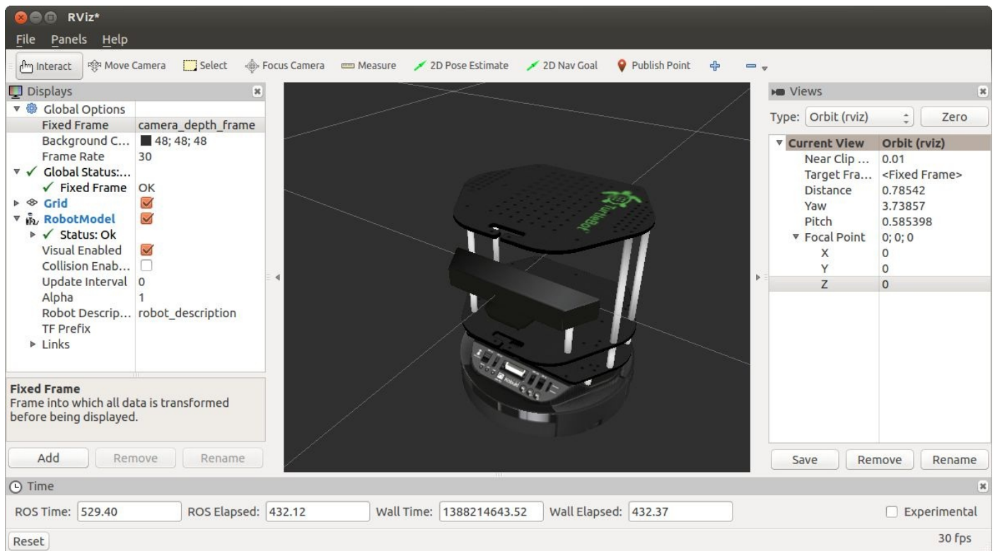
Figure 8-8. A Turtlebot model added to rviz
