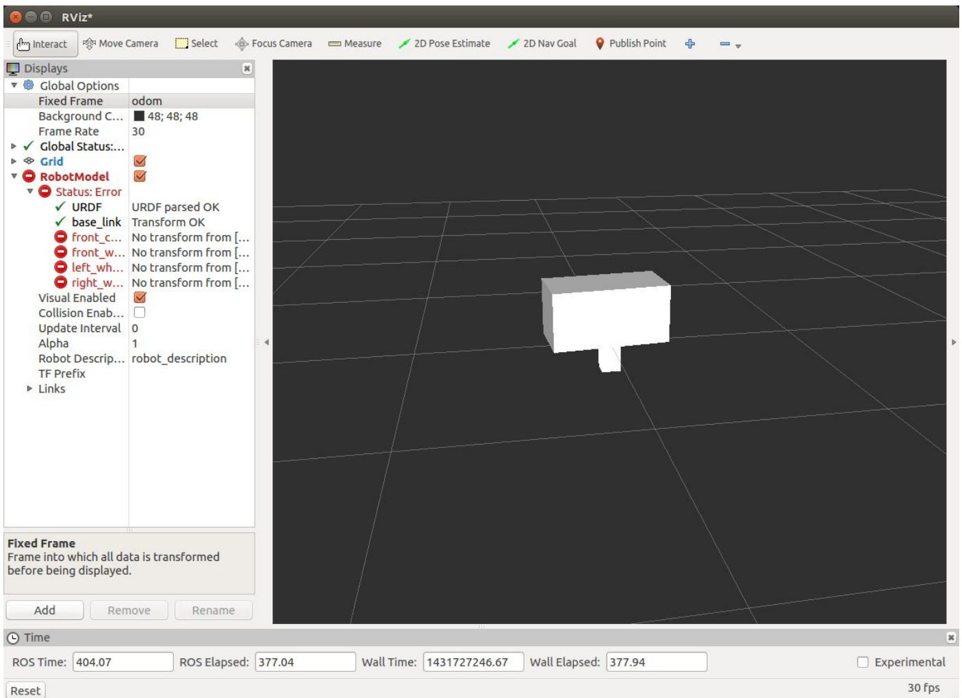
Figure 17-1. Visualization of the TortoiseBot with missing transforms
