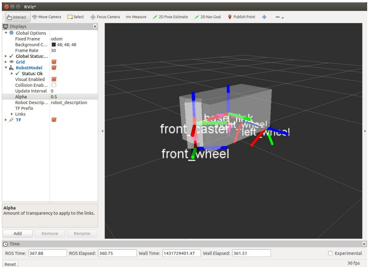
Figure 17-3. Visualization of the TortoiseBot with transforms visualized
