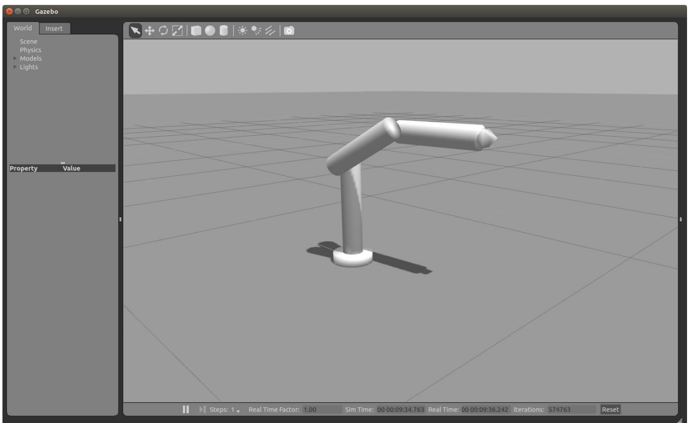
Figure 18-6. CougarBot arm moved to a new configuration
