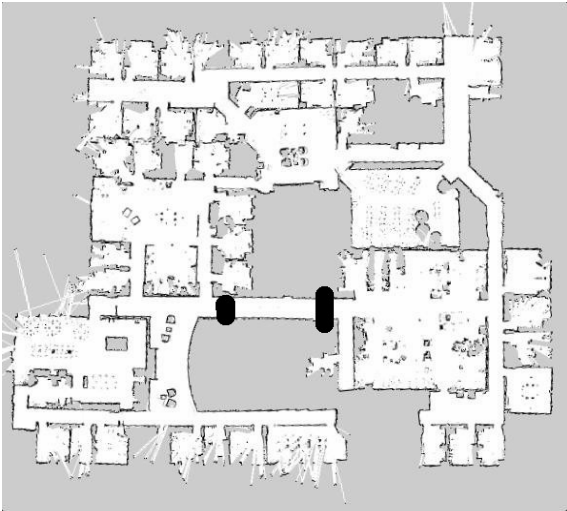
Figure 9-2. A hand-modified map — black lines were added to stop the robot from planning paths down the corridor in the middle of the map
