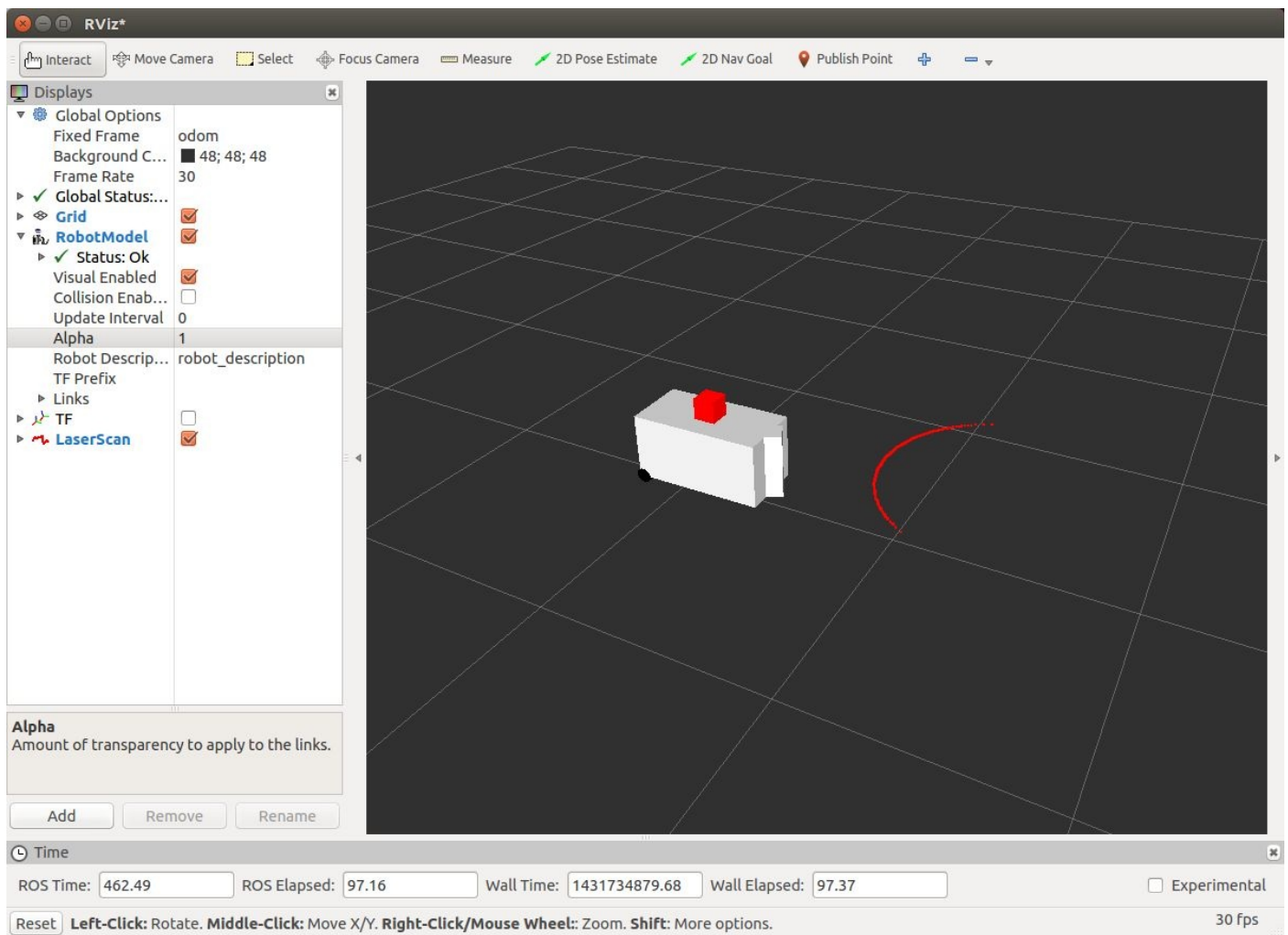
Figure 17-5. Visualization of laser scans from the TortoiseBot
