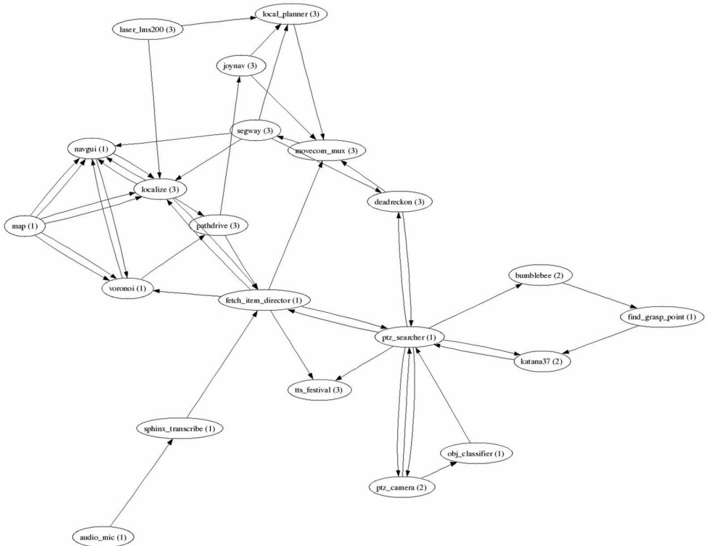
Figure 2-8. ROS graph of a fetch-an-item robot
