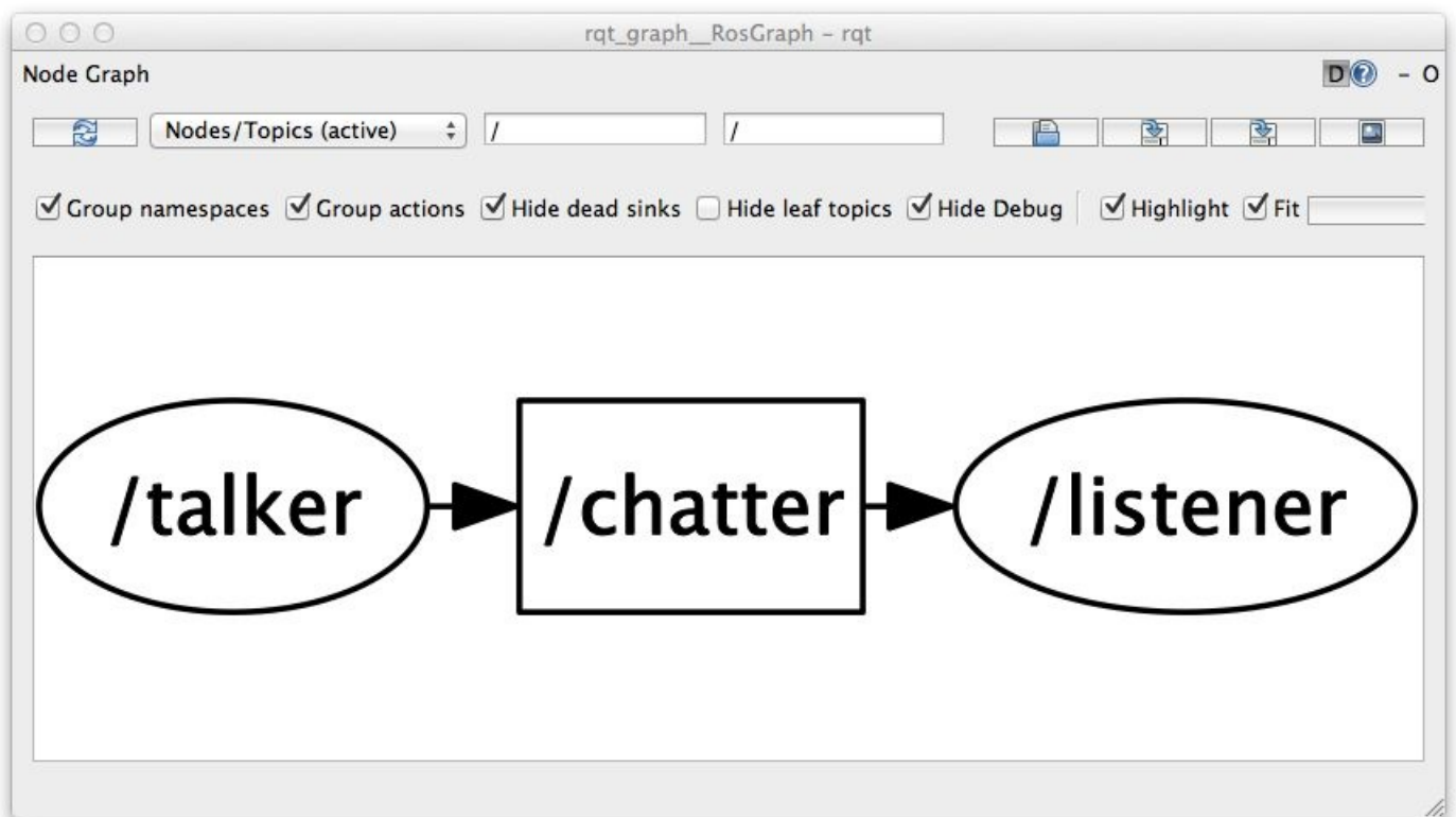
Figure 21-3. The rqt_graph GUI shows the current state of nodes and topics in a running ROS system
