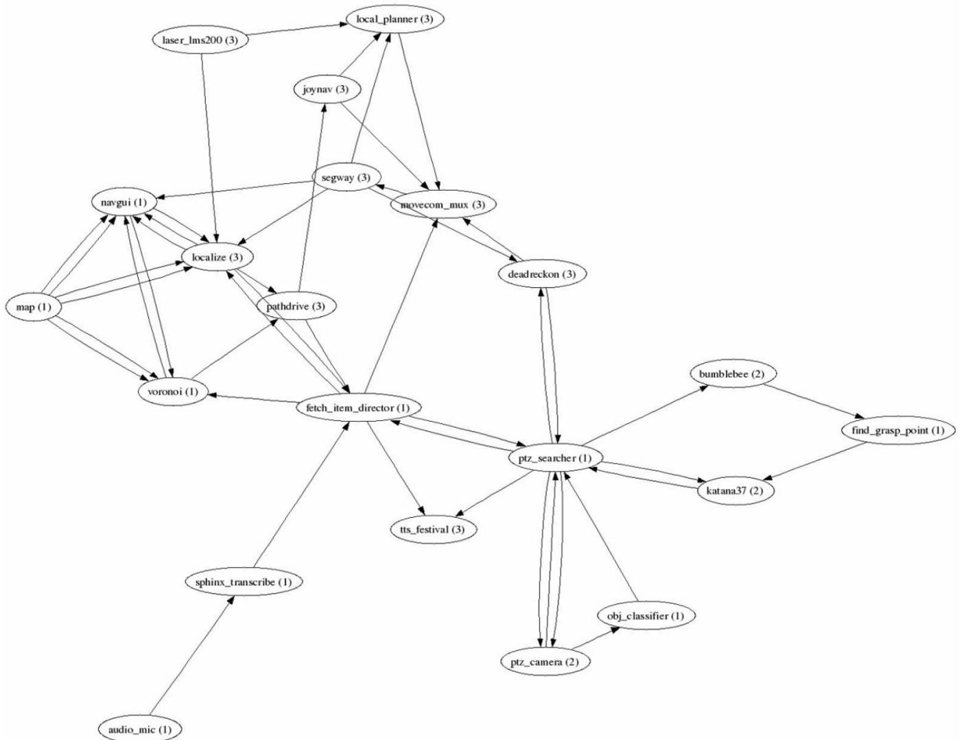
Figure 2-1. ROS graph of a fetch-an-item robot — nodes in the graph represent individual programs; edges represent message streams communicating sensor data, actuator commands, planner states, intermediate representations, and so on
