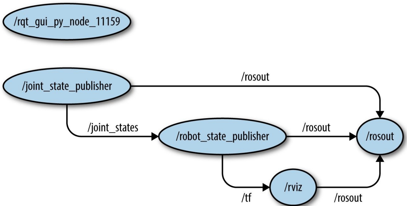
Figure 16-5. rqt_graph view of the nodes involved in visualizing and actuating the TortoiseBot model
