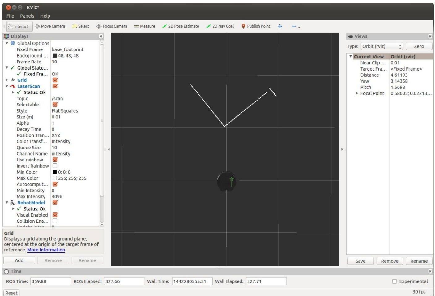
Figure 7-3. A bird's-eye view of the same scene as Figure 7-2, rendering the simulated laser scan extracted from the simulated Kinect data of the Turtlebot — the object directly in front of the robot is visible, but the object to its right is mostly out of view
