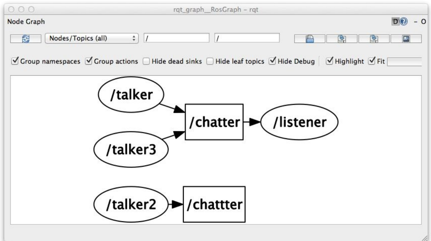
Figure 21-6. Two nodes are publishing to a subscriber, but they disagree on the message type; further investigation is needed
