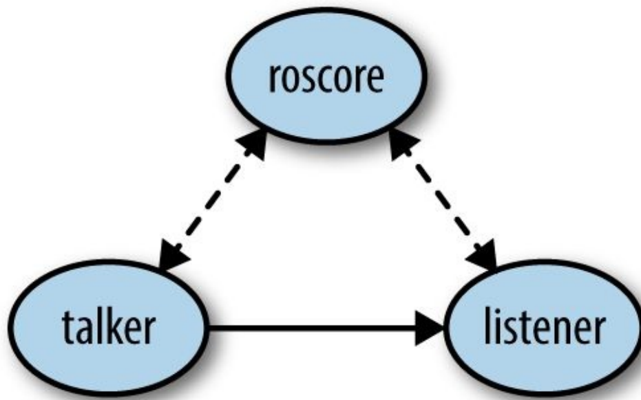
Figure 2-2. roscore connects only ephemeraly to the other nodes in the system
