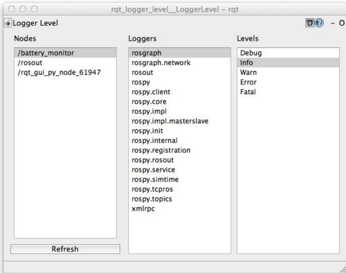
Figure 21-1. The rqt_logger_level GUI allows you to change the debugging logger level of any running ROS node
