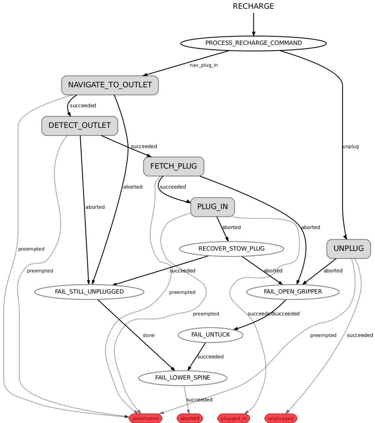
Figure 13-1. State machine for the PR2 robot to plug into an electrical outlet, generated by the smach_viewer node
