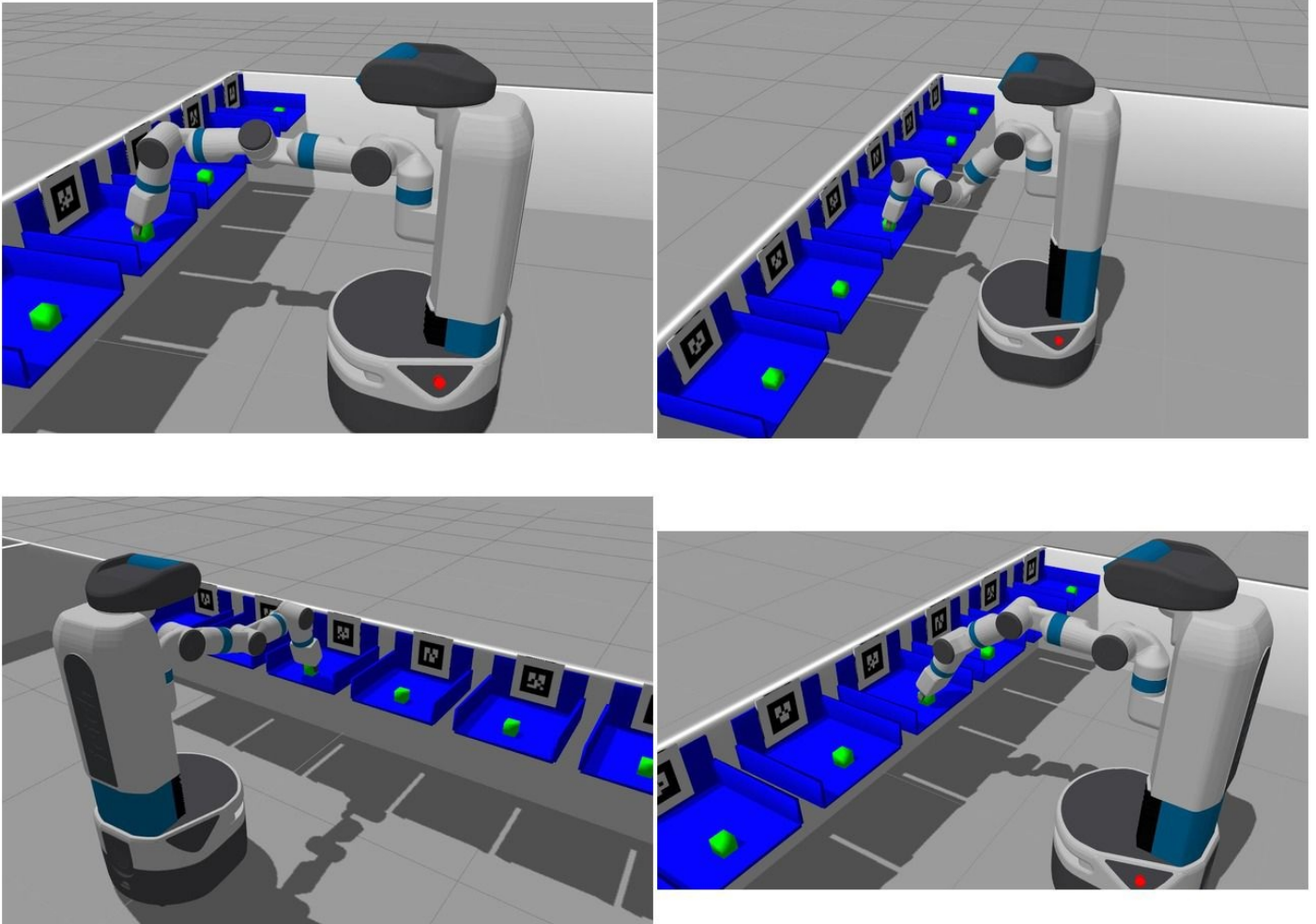
Figure 14-12. Various grasps found by MoveIt for different alignments of the robot with respect to the bin
