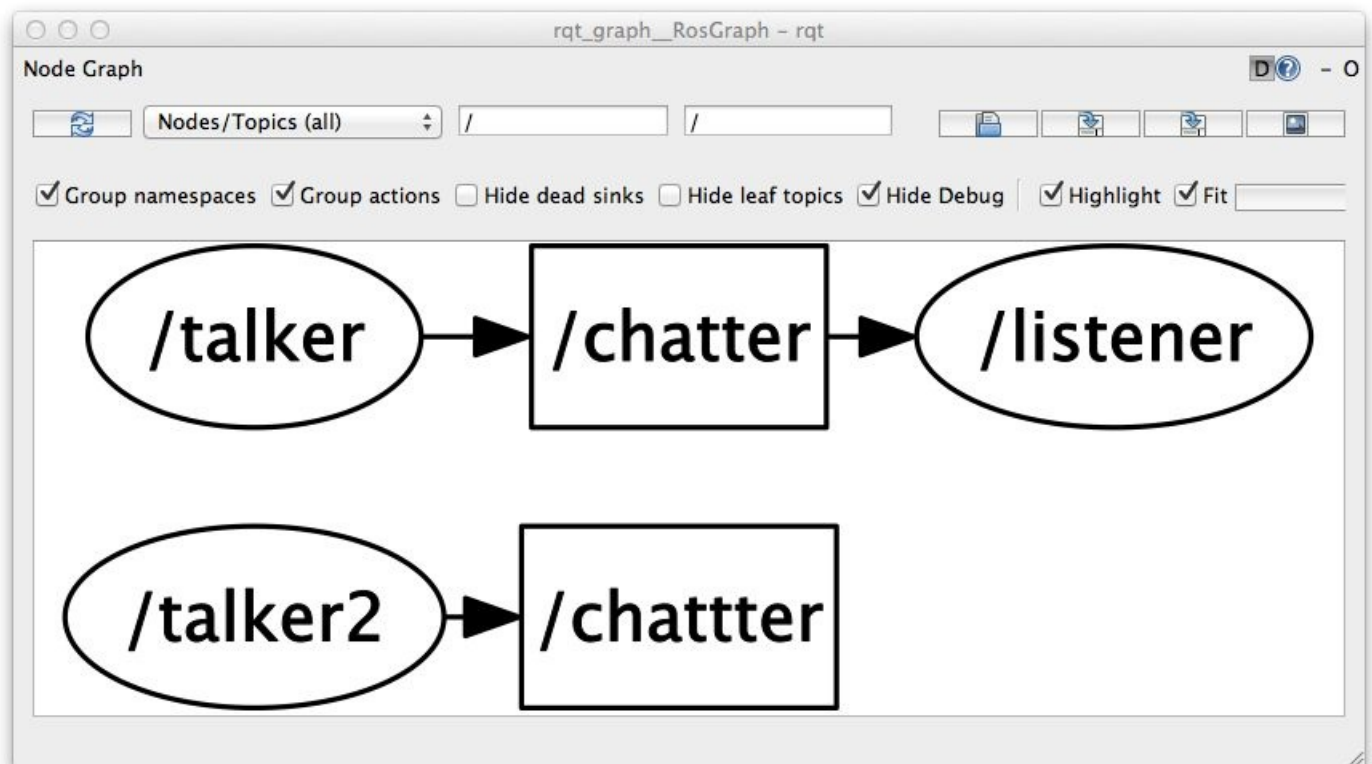
Figure 21-5. A missing connection caused by a misspelled topic name can be seen clearly in rqt_graph
