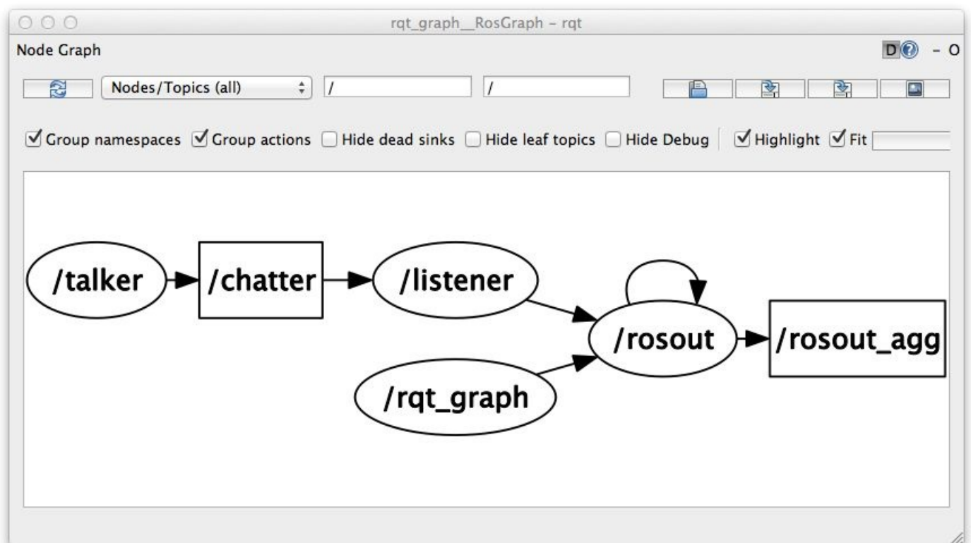
Figure 21-4. The options in rqt_graph allow you to reveal more or less about a running ROS system
