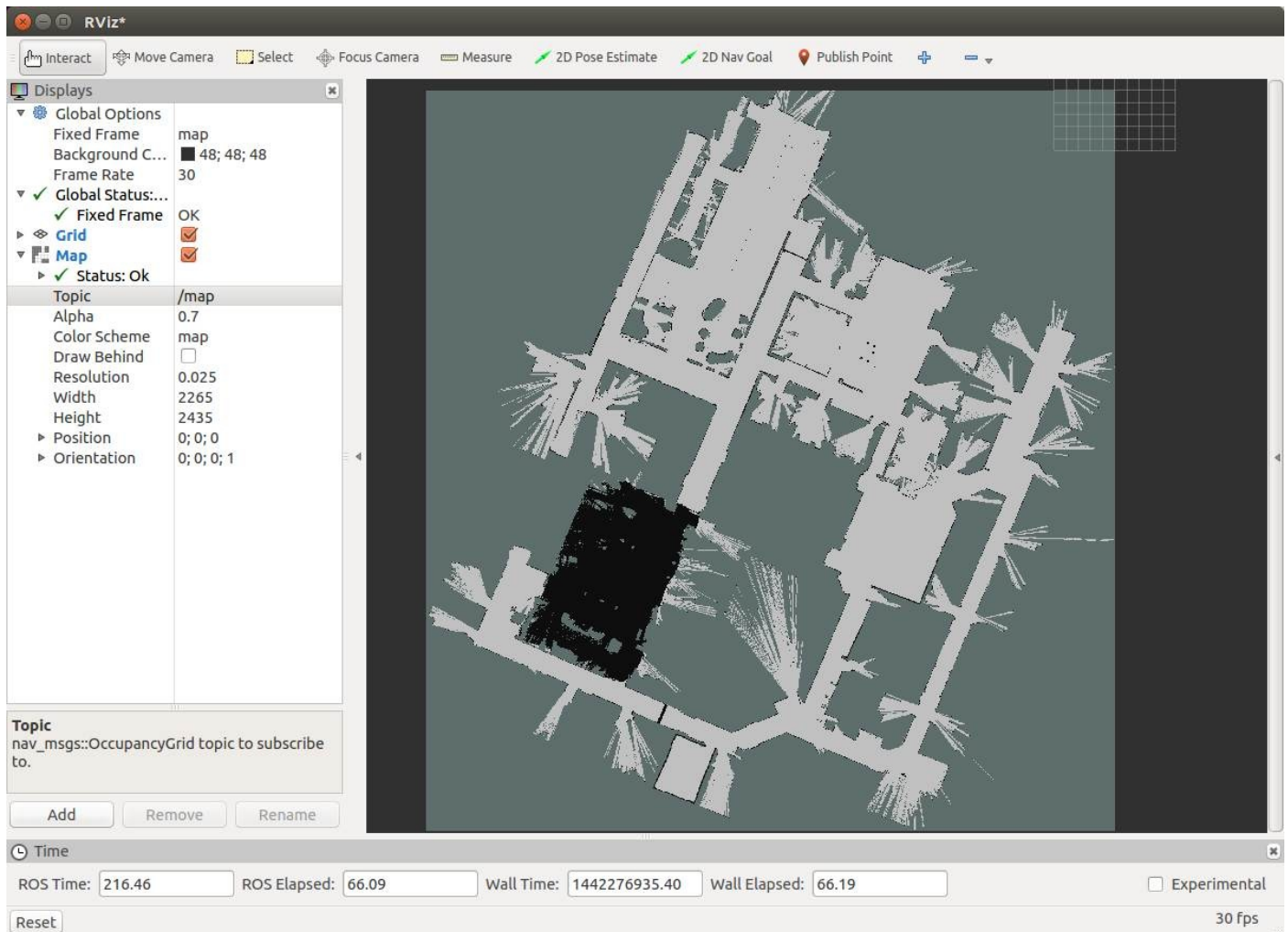
Figure 17-8. The static map displayed in rviz
